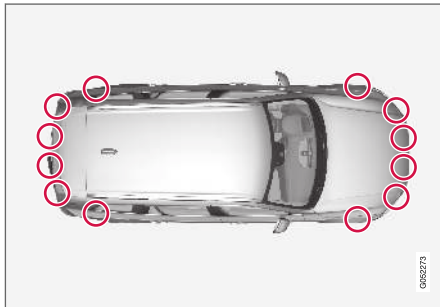
Location of the Park Assist sensors 130 .
