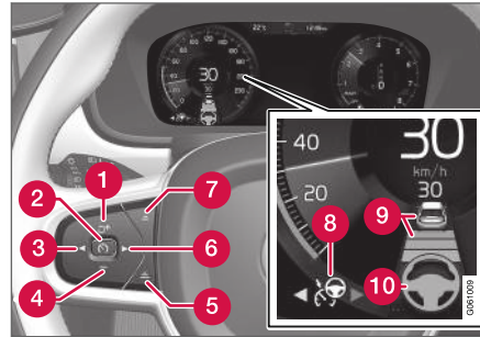
Function buttons and symbols 61 .
