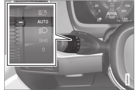
Lighting ring in AUTO position.
