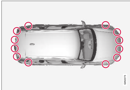
Location of the Park Assist sensors 129 .
