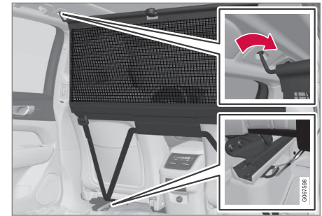
Fremre montering.
