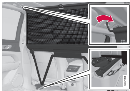
Front mounting.
