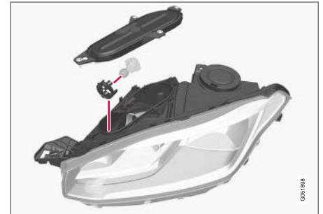
Venstre frontlys.
